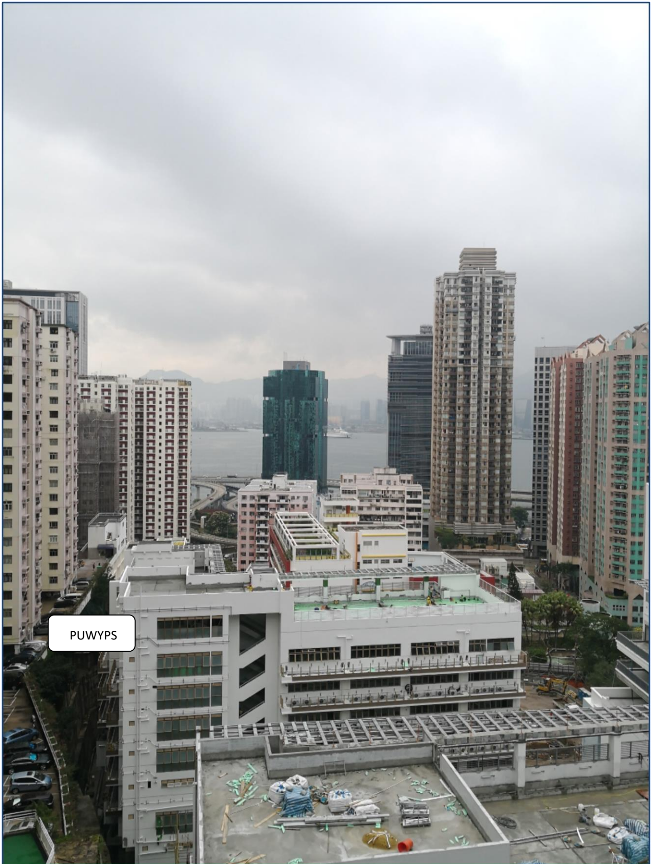
Main Building – Construction works substantially completed. Installation of metal louvers and canopy on 7/F, railings to AC platforms and interior works in progress.
